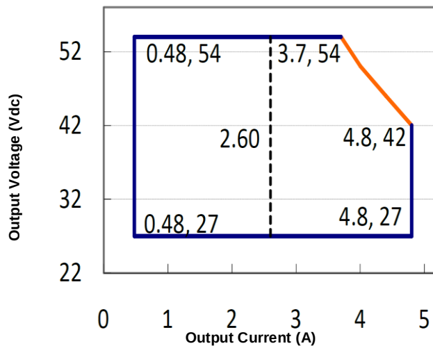
Figure 2: Typical V-I Characteristic Curve (LTA200X-054C)
