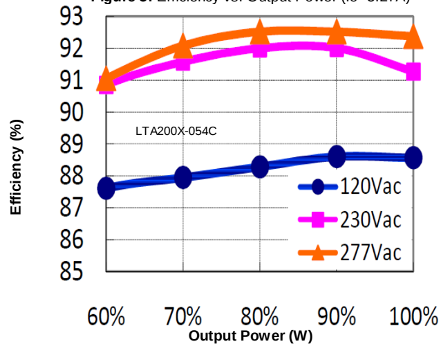
Figure 7: Efficiency vs. Output Power ( I_o=3.70A )
