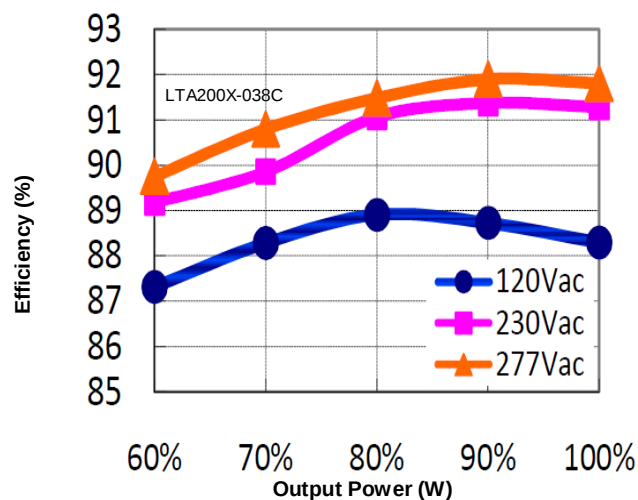
Figure 5: Efficiency vs. Output Power ( I_o=5.27A )
