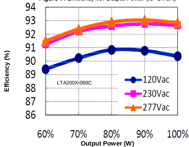
Figure 9: Efficiency vs. Output Power ( I_o=2.95A )
