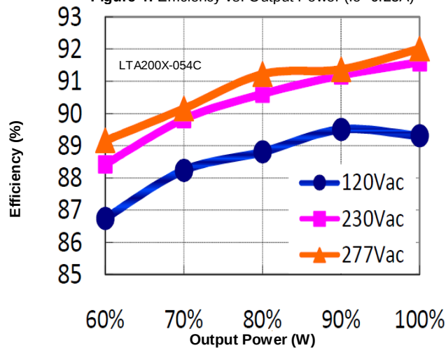
Figure 6: Efficiency vs. Output Power ( I_o=4.80A )
