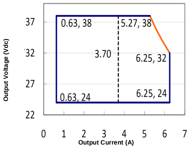
Figure 1: Typical V-I Characteristic Curve (LTA200X-038C)
