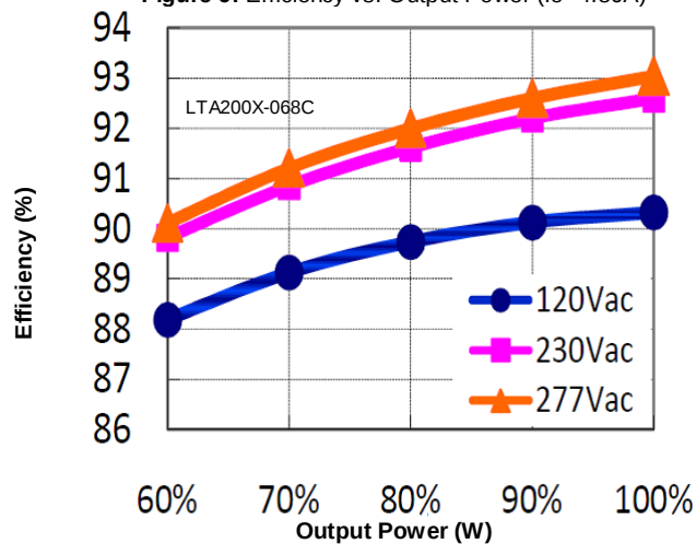
Figure 8: Efficiency vs. Output Power ( I_o=3.60A )
