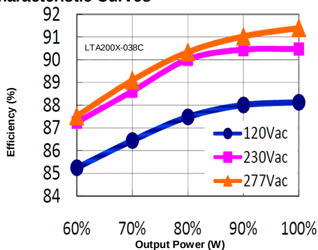
Figure 4: Efficiency vs. Output Power ( I_o=6.25A )
