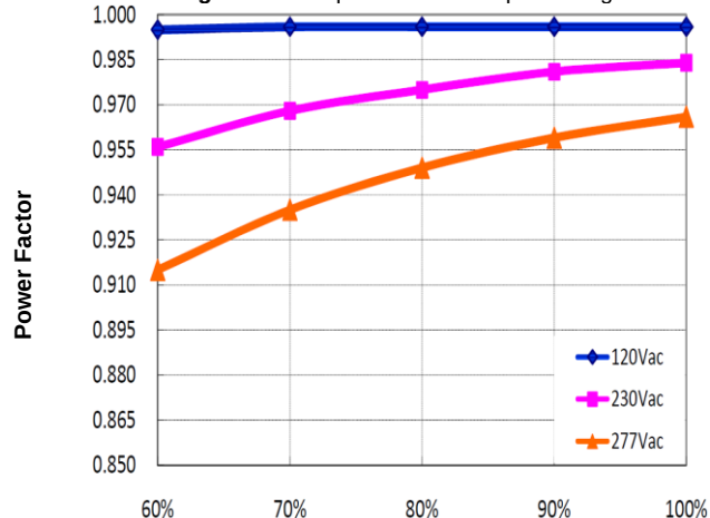
Figure 13: Power Factor vs. Output Power
