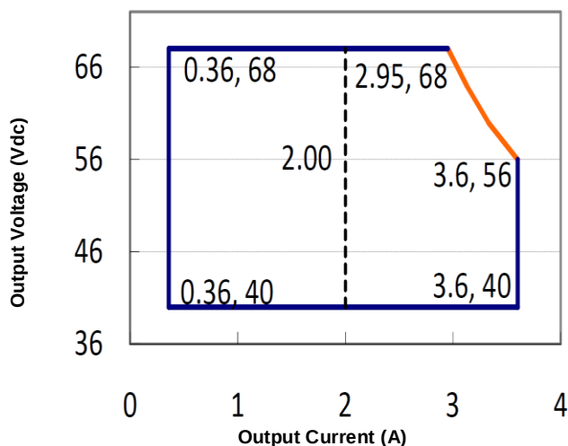
Figure 3: Typical V-I Characteristic Curve (LTA200X-068C)
